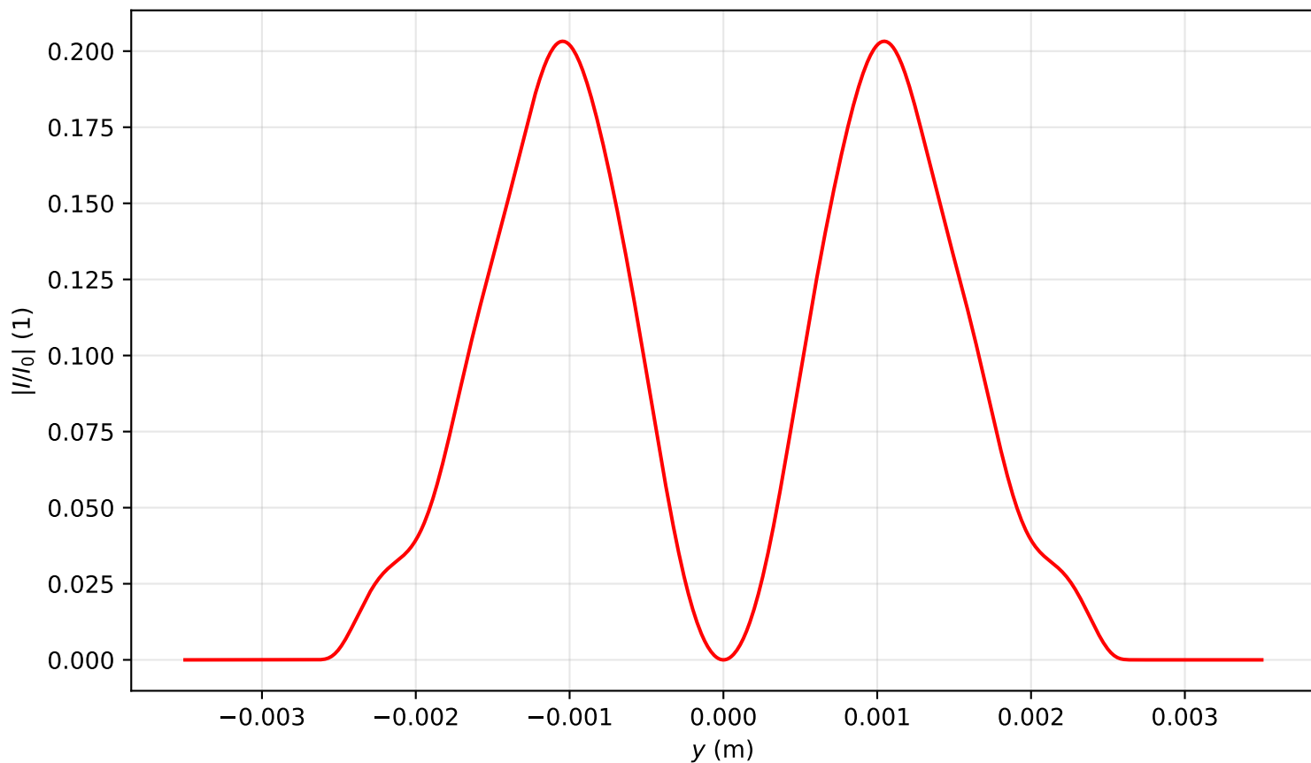
Intensity profile I(x=0, y, z=3.901)/I_0 , P_{in}=1.0P_{cr} , artificial time
